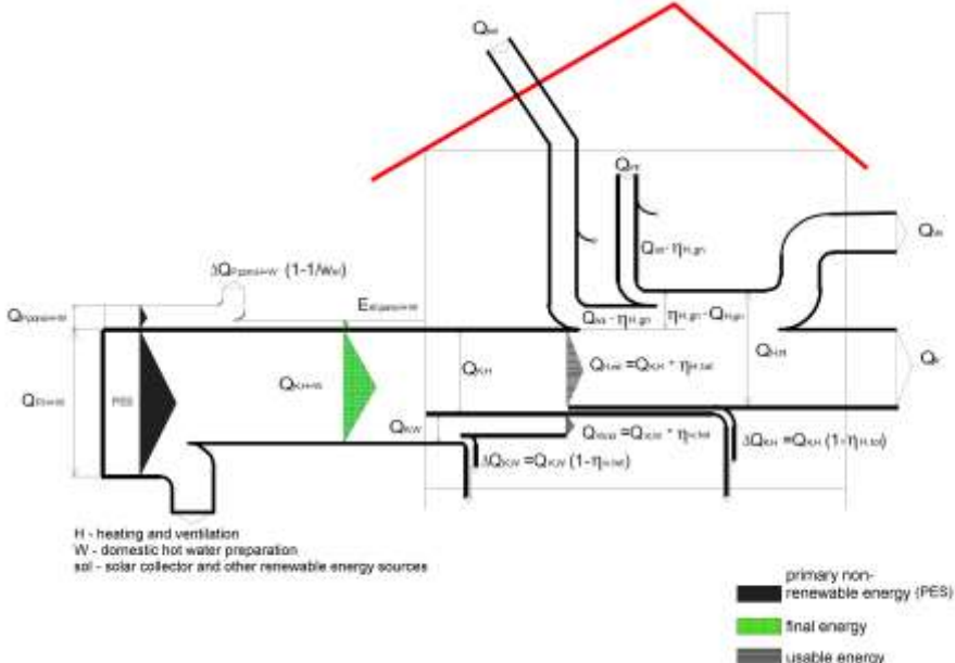
Figure 1 – Sankey’s diagram – balance of primary, final and utility energy and its flows for heating and ventilation and preparation of hot water in a building with renewable energy sources [16]
