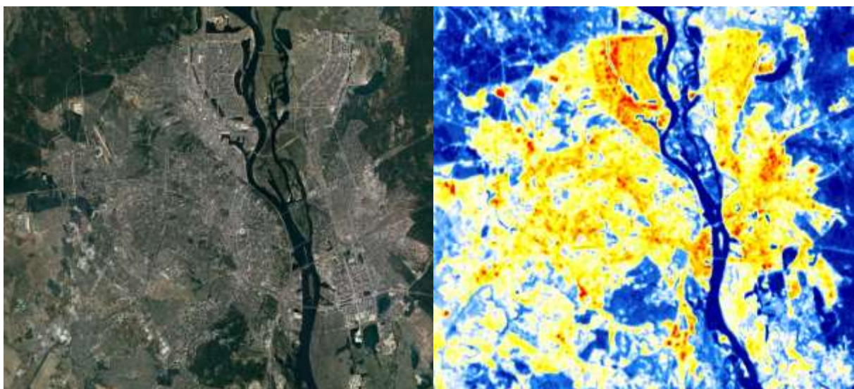
Figure 1 – Kyiv under the scope of the Landsat 8 satellite (summer, 2022)
